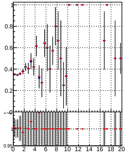
Fake rate vs. —●— DQM_TT_mkFit-DQM_init_orig —●— DQM_TT_mkFit-DQM_init_modi
