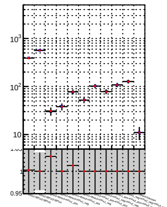
N of reco track vs. \chi^2 — DQM TT mkFit-DQM_init_orig — DQM TT mkFit-DQM_init_modi
