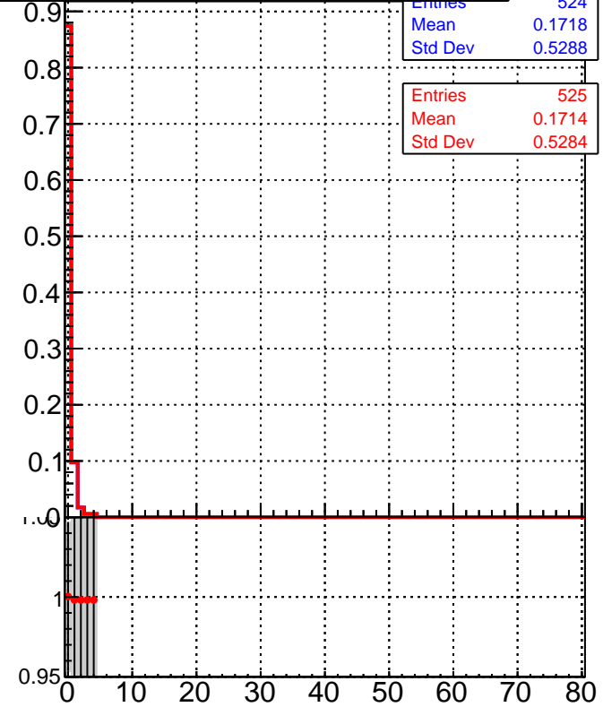
■ DQM_TT_mkFit-DQM_init_orig ● DQM_TT_mkFit-DQM_init_modi
