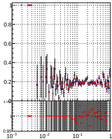
—•— DQM_TT_mkFit-DQM_init_orig —•— DQM_TT_mkFit-DQM_init_modi
