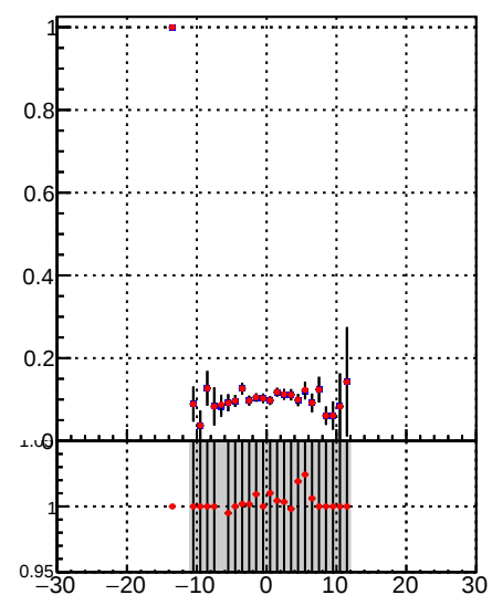
Fake rate vs d —•— DQM_TT_mkFit-DQM_init_orig —•— DQM_TT_mkFit-DQM_init_modi
