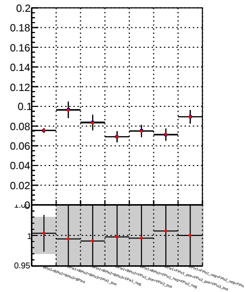
Fake rate vs. — DQM_TT_mkFit-DQM_init_orig — DQM_TT_mkFit-DQM_init_modi
