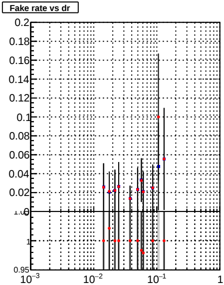
Fake rate vs dr Legend: DQM_TT_mkFit-DQM_init_orig DQM_TT_mkFit-DQM_init_modi
