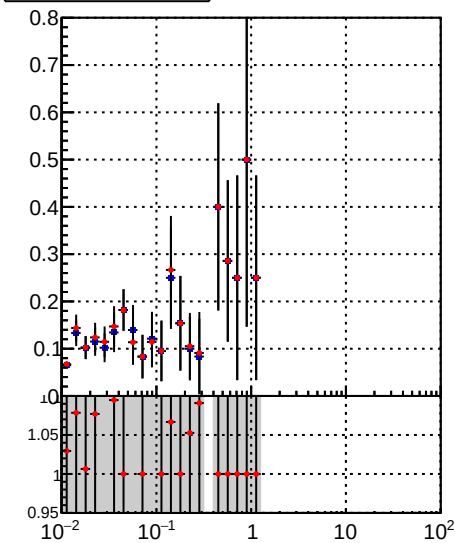
—•— DQM_TT_mkFit-DQM_init_orig —•— DQM_TT_mkFit-DQM_init_modi
