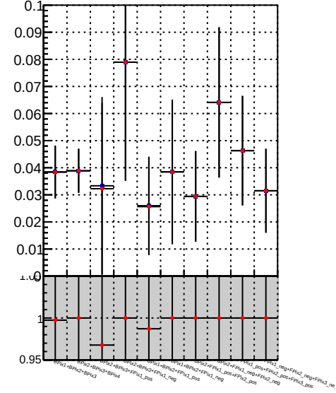
Fake rate vs. —•— DQM TT mkFit-DQM_init_orig —•— DQM TT mkFit-DQM_init_modi
