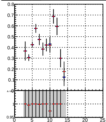
Legend: DQM_TT_mkFit-DQM_init_orig (blue line with dots), DQM_TT_mkFit-DQM_init_modi (red line with dots)
