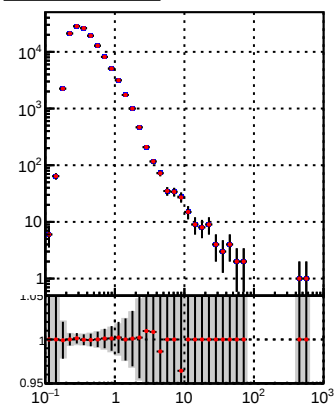
—●— DQM_TT_mkFit-DQM_init_orig —●— DQM_TT_mkFit-DQM_init_modi
