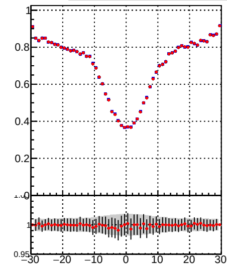
—•— DQM_TT_mkFit-DQM_init_orig —•— DQM_TT_mkFit-DQM_init_modi
