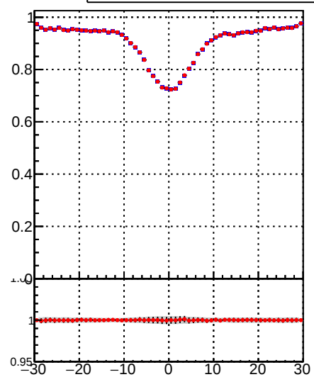
—•— DQM_TT_mkFit-DQM_init_orig —•— DQM_TT_mkFit-DQM_init_modi
