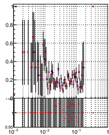
—●— DQM_TT_mkFit-DQM_init_orig —●— DQM_TT_mkFit-DQM_init_modi
