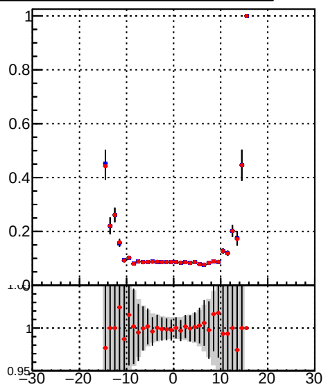
Efficiency vs. vert r Legend: — DQM_TT_mkFit-DQM_init_orig — DQM_TT_mkFit-DQM_init_modi
