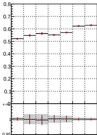
Fake rate vs. \bullet DQM_TT_mkFit-DQM_init_orig \bullet DQM_TT_mkFit-DQM_init_modi
