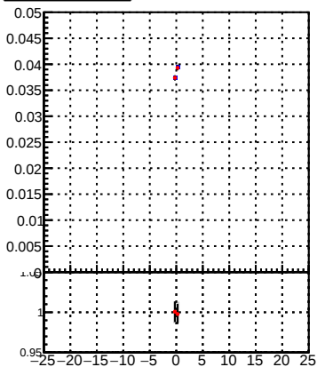
—●— DQM_TT_mkFit-DQM_init_orig —●— DQM_TT_mkFit-DQM_init_modi
