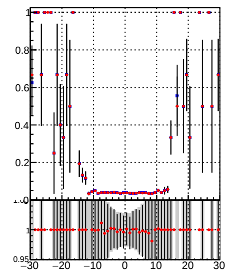
Fake rate vs d —•— DQM_TT_mkFit-DQM_init_orig —•— DQM_TT_mkFit-DQM_init_modi
