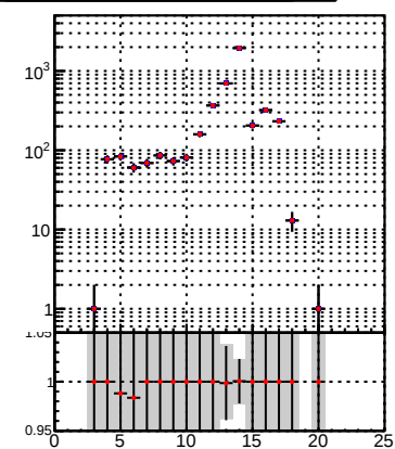
N of associated tracks (simToReco) vs hit (zoomed)
