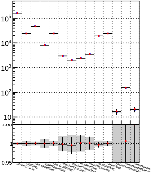
Number —●— DQM_TT__mkFit-DQM_init_modi
