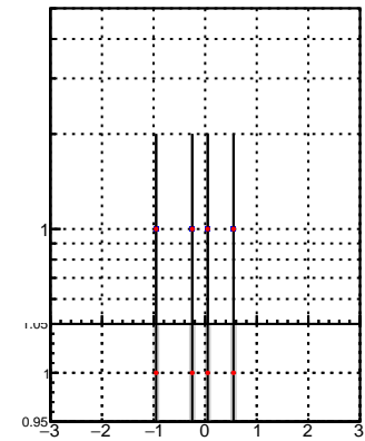
N of reco track vs \eta vs \eta —•— DQM TT mkFit-DQM_init_orig —•— DQM TT mkFit-DQM_init_modi
