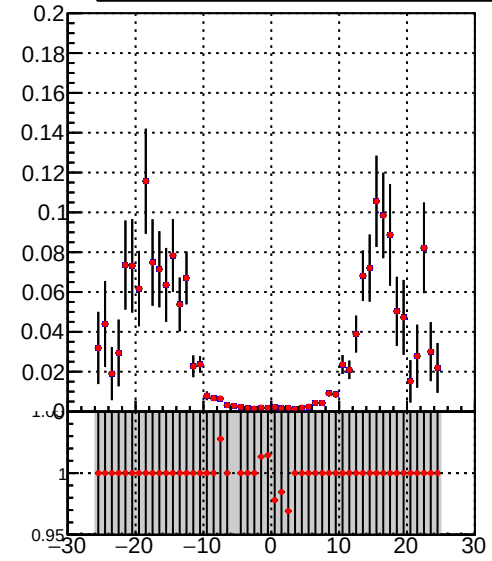
Efficiency vs. sim PV z Legend: DQM_TT_mkFit-DQM_init_orig (Blue line with markers) DQM_TT_mkFit-DQM_init_modi (Red line with markers)
