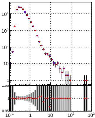
—●— DQM_TT_mkFit-DQM_init_orig —●— DQM_TT_mkFit-DQM_init_modi
