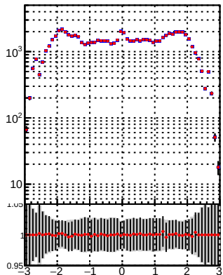
—●— DQM_TT_mkFit-DQM_init_orig —●— DQM_TT_mkFit-DQM_init_modi
