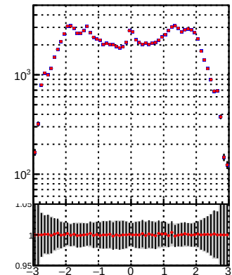
—●— DQM_TT_mkFit-DQM_init_orig —●— DQM_TT_mkFit-DQM_init_modi
