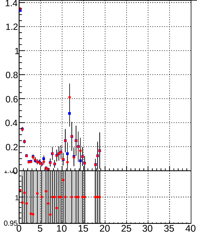
K_S^0 tracking fake rate vs p_T and \eta Legend: \blacksquare DQM_TT_mkFit-DQM_init_orig \bullet DQM_TT_mkFit-DQM_init_modi
