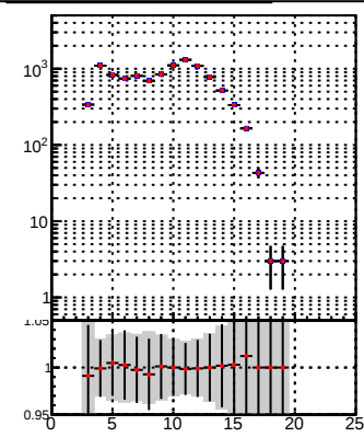
—•— DQM_TT_mkFit-DQM_init_orig —•— DQM_TT_mkFit-DQM_init_modi
