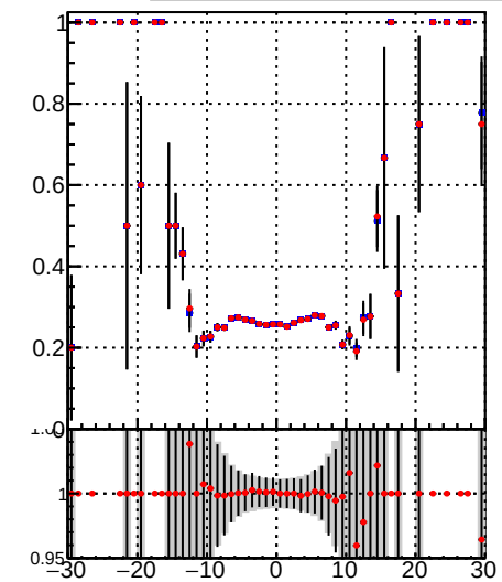
—•— DQM_TT_mkFit-DQM_init_orig —•— DQM_TT_mkFit-DQM_init_modi
