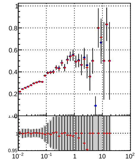
—•— DQM_TT_mkFit-DQM_init_orig —•— DQM_TT_mkFit-DQM_init_modi
