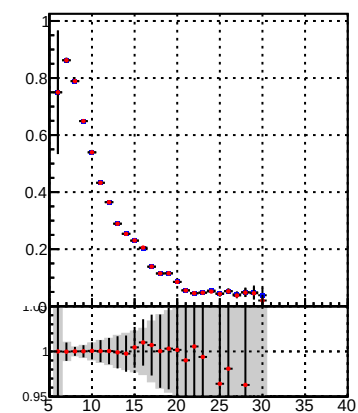
Fake rate vs hit Legend: DQM_TT_mkFit-DQM_init_orig (blue line), DQM_TT_mkFit-DQM_init_modi (red line)
