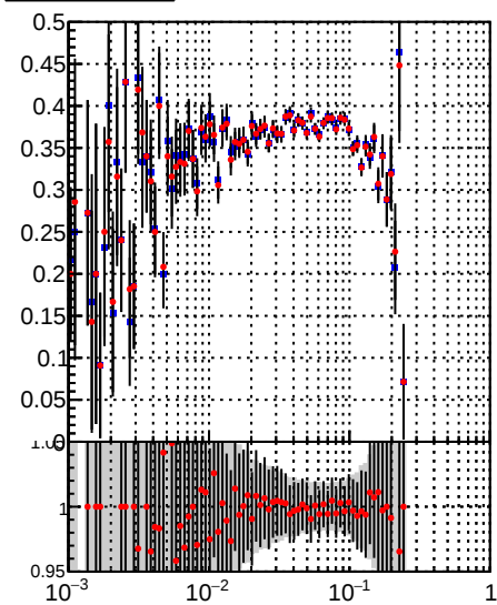
■ DQM_TT_mkFit-DQM_init_orig ● DQM_TT_mkFit-DQM_init_modi
