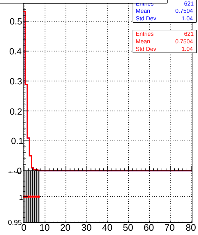
Legend: DQM_TT_mkFit-DQM_init_orig (blue line with squares) DQM_TT_mkFit-DQM_init_modi (red line with circles)
