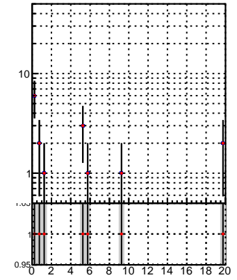
N of associated (recoToSim) looper tracks vs normalized \chi^2
