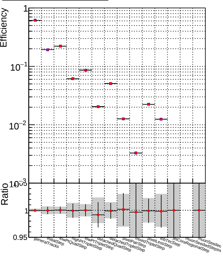
DQM_TT_mkFit-DQM_old132 DQM_TT_mkFit-DQM_new132
