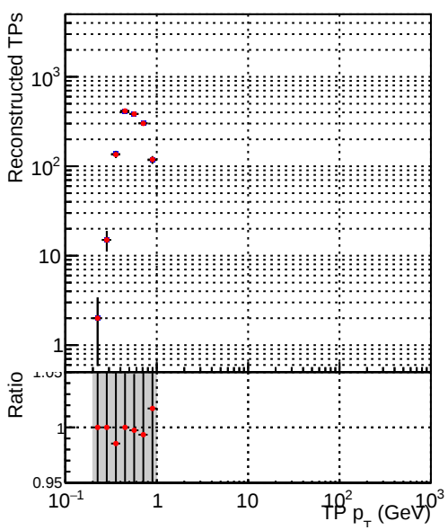
—•— DQM_TT__mkFit-DQM_old132 —•— DQM_TT__mkFit-DQM_new132
