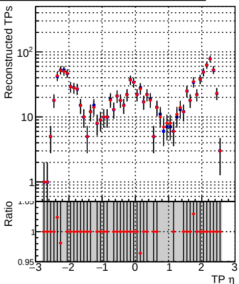
—•— DQM_TT__mkFit-DQM_old132 —•— DQM_TT__mkFit-DQM_new132
