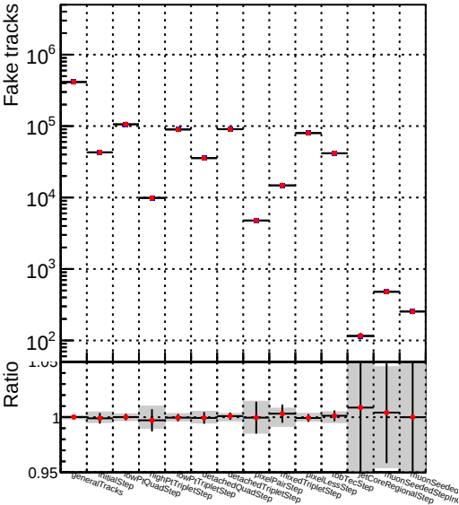
Number —●— DQM_TT_mkFit-DQM_new132
