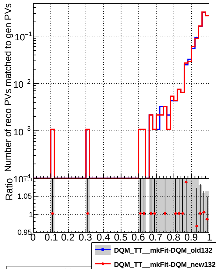
RecoPVAssoc2GenPVmatched_missing
