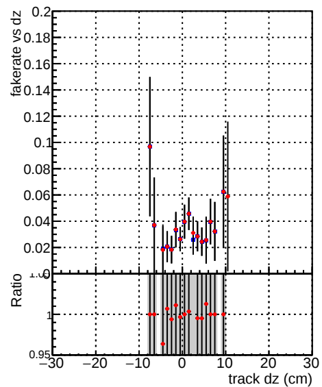
Fake rate vs dz —●— DQM_TT_mkFit-DQM_old132 —●— DQM_TT_mkFit-DQM_new132
