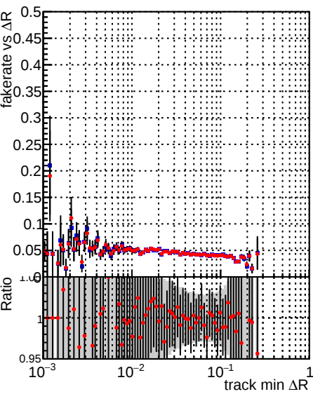
Fake rate vs ΔR(track, jet) DQM_TT_mkFit-DQM_old132 DQM_TT_mkFit-DQM_new132
