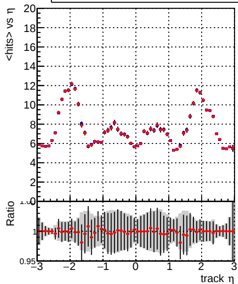
mean hit — DQM_TT_mkFit-DQM_old132 — DQM_TT_mkFit-DQM_new132
