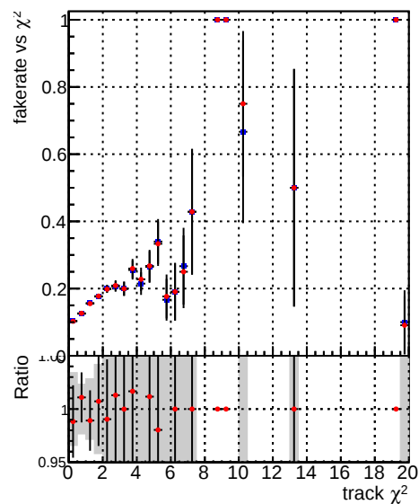
Fake rate vs. —●— DQM TT mkFit-DQM_old132 —●— DQM TT mkFit-DQM_new132
