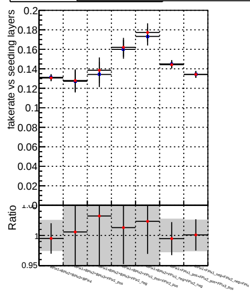
Fake rate vs. —●— DQM TT mkFit-DQM_old132 —●— DQM TT mkFit-DQM_new132
