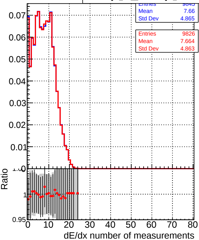
DQM_TT_mkFit-DQM_old132 DQM_TT_mkFit-DQM_new132
