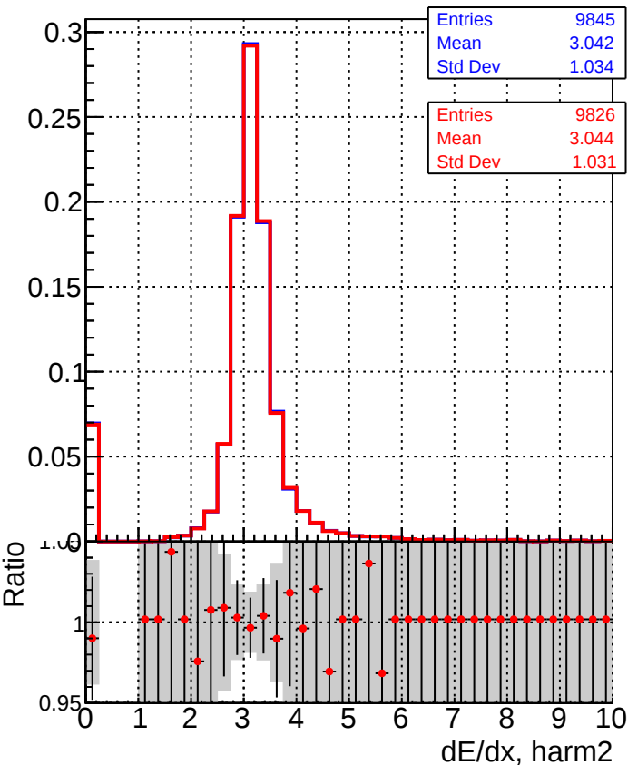
DQM_TT_mkFit-DQM_old132 DQM_TT_mkFit-DQM_new132
