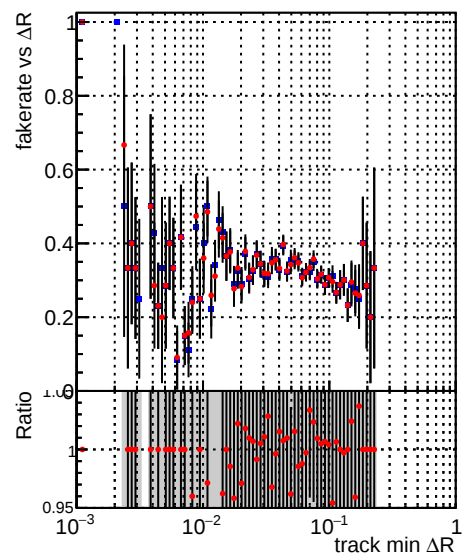
—•— DQM_TT_mkFit-DQM_old132 —•— DQM_TT_mkFit-DQM_new132
