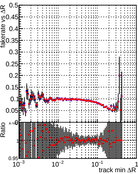
Fake rate vs \Delta R (track, jet) DQM_TT_mkFit-DQM_old132 DQM_TT_mkFit-DQM_new132
