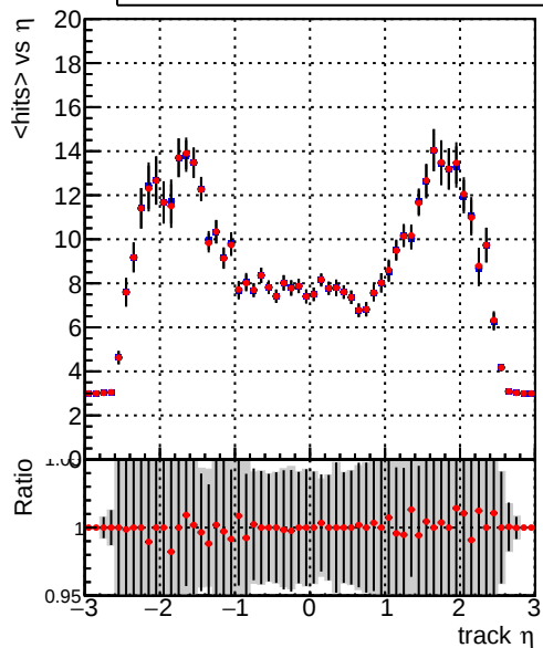
mean hits — DQM_TT_mkFit-DQM_old132 — DQM_TT_mkFit-DQM_new132
