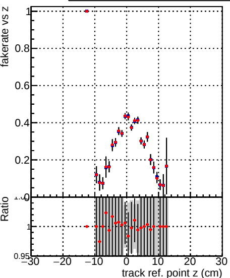
Fake rate vs verpos DQM_TT_mkFit-DQM_old132 DQM_TT_mkFit-DQM_new132
