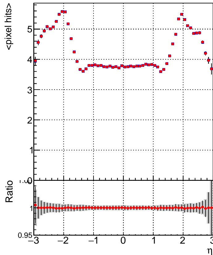
■ DQM_TT_mkFit-DQM_old132 ■ DQM_TT_mkFit-DQM_new132
