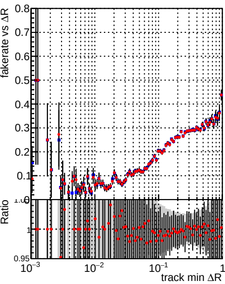
Fake rate vs \Delta R(\text{track, jet}) Legend: DQM_TT_mkFit-DQM_old132 DQM_TT_mkFit-DQM_new132
