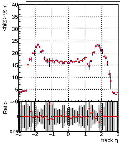
— DQM_TT_mkFit-DQM_old132 — DQM_TT_mkFit-DQM_new132
