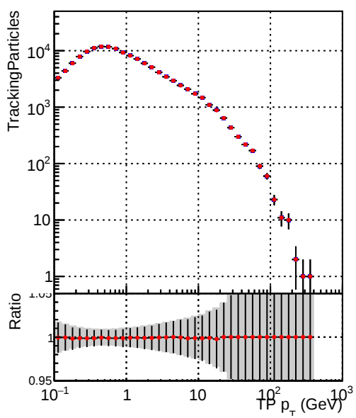
Legend: DQM_TT_mkFit-DQM_old132 (blue line with dots), DQM_TT_mkFit-DQM_new132 (red line with stars)
