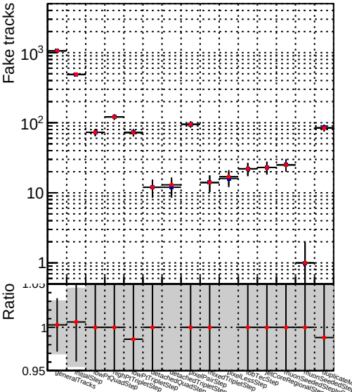
Number —●— DQM_TT__mkFit-DQM_new132
