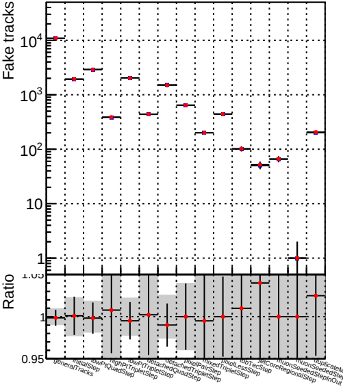
Number —●— DQM_TT_mkFit-DQM_new132
