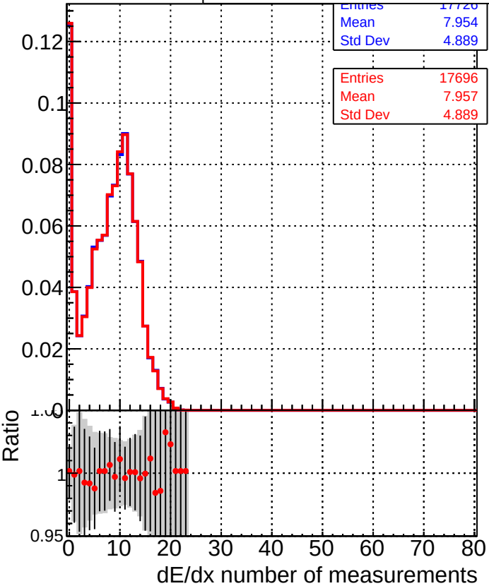
■ DQM_TT_mkFit-DQM_old132 ● DQM_TT_mkFit-DQM_new132
