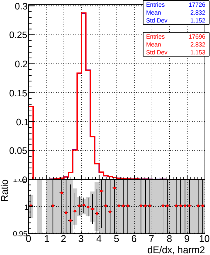
■ DQM_TT_mkFit-DQM_old132 ● DQM_TT_mkFit-DQM_new132
